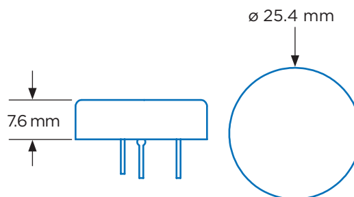
Cell Drawing
